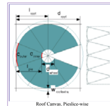
Roof Canvas, Pieslice-wise
